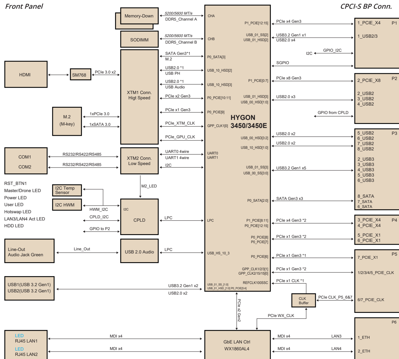
Front Panel
