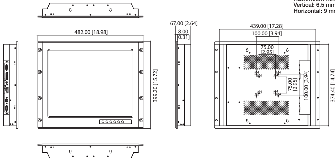
Panel Cutout Dimensions: 441 x 376.4 mm (17.36 x 14.81 in)
