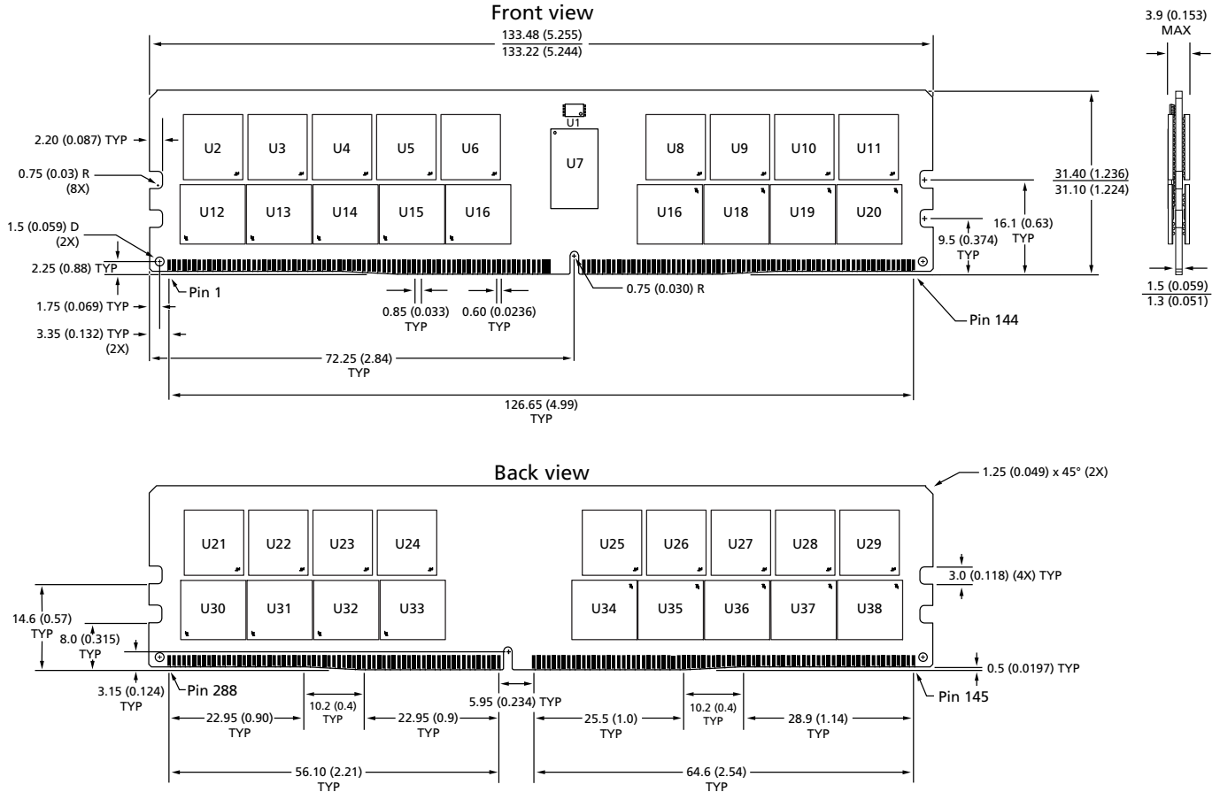
Figure 3: 288-Pin DDR4 RDIMM (R/C-B3)
